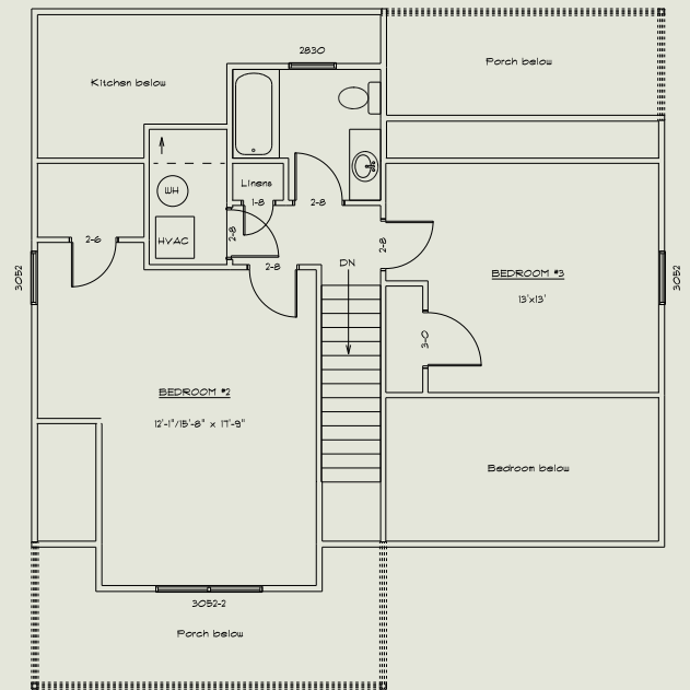
The Paige Second Floor Plan
