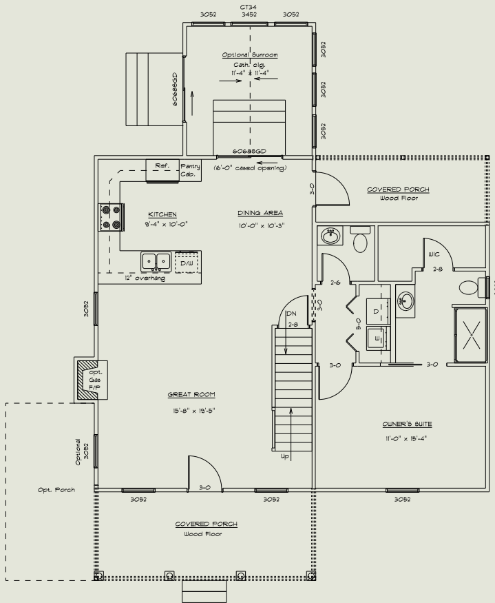
The Paige First Floor Plan
