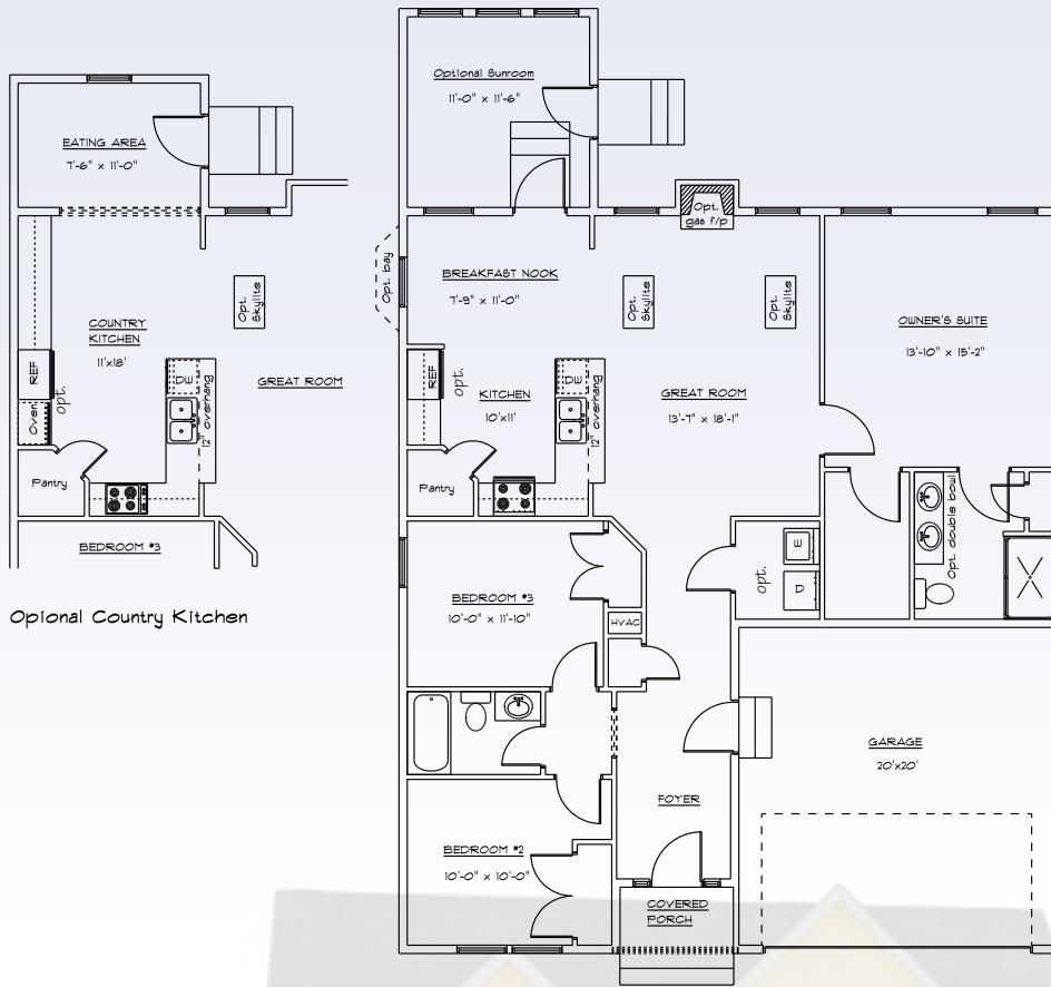
Standard Jackson Floor Plan
