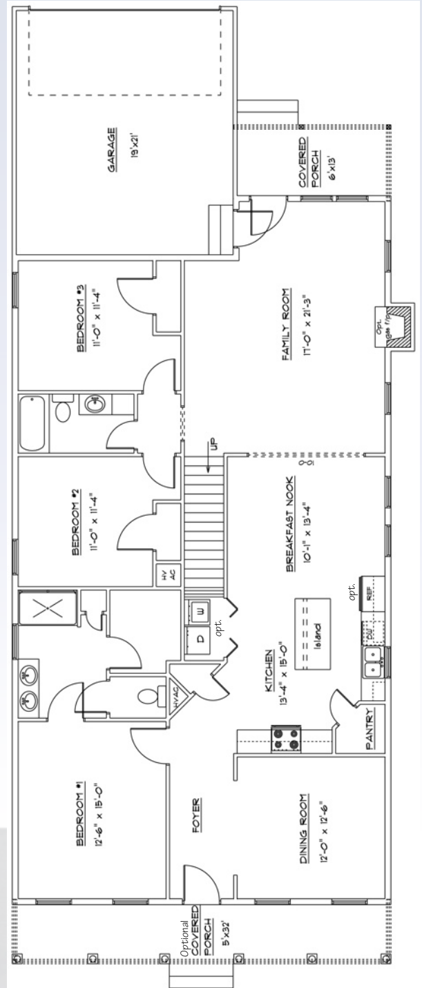
FIRST FLOOR PLAN OPTIONAL FEATURES MAY BE SHOWN
