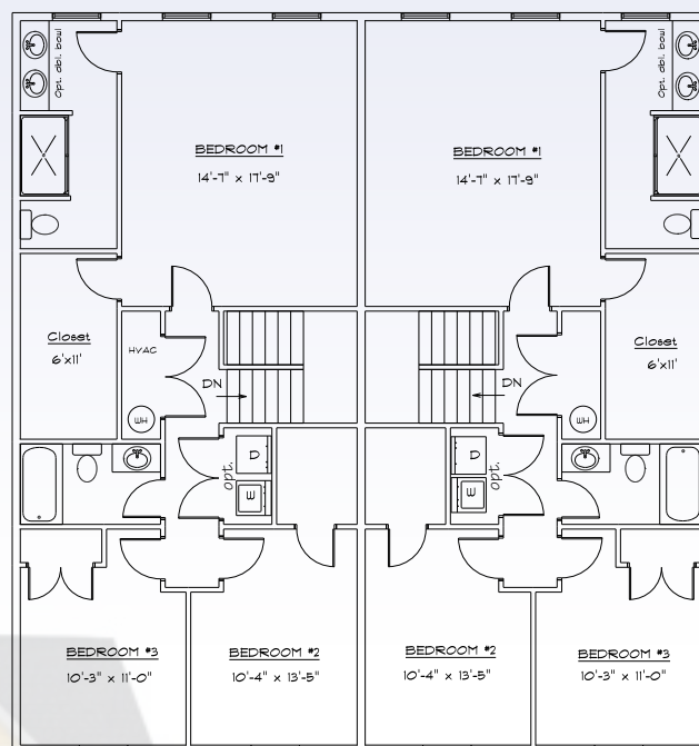
SECOND FLOOR PLAN (TWO UNITS SHOWN)
