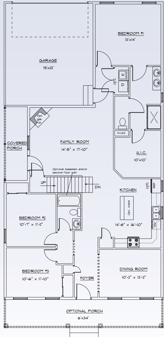
The Tanner Enlarged Floor Plan
