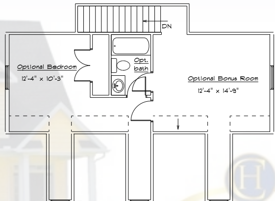
The Tanner Second Floor Plan (Elevation 'B')
