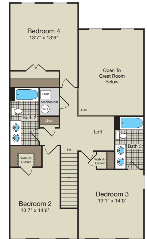
SECOND FLOOR Option 3
